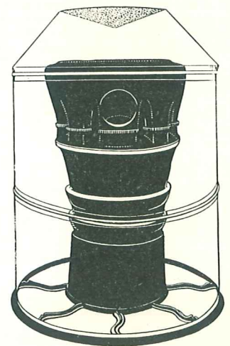
Diagram to show gradual flare of castings—also relation of these castings to the warm air chamber
